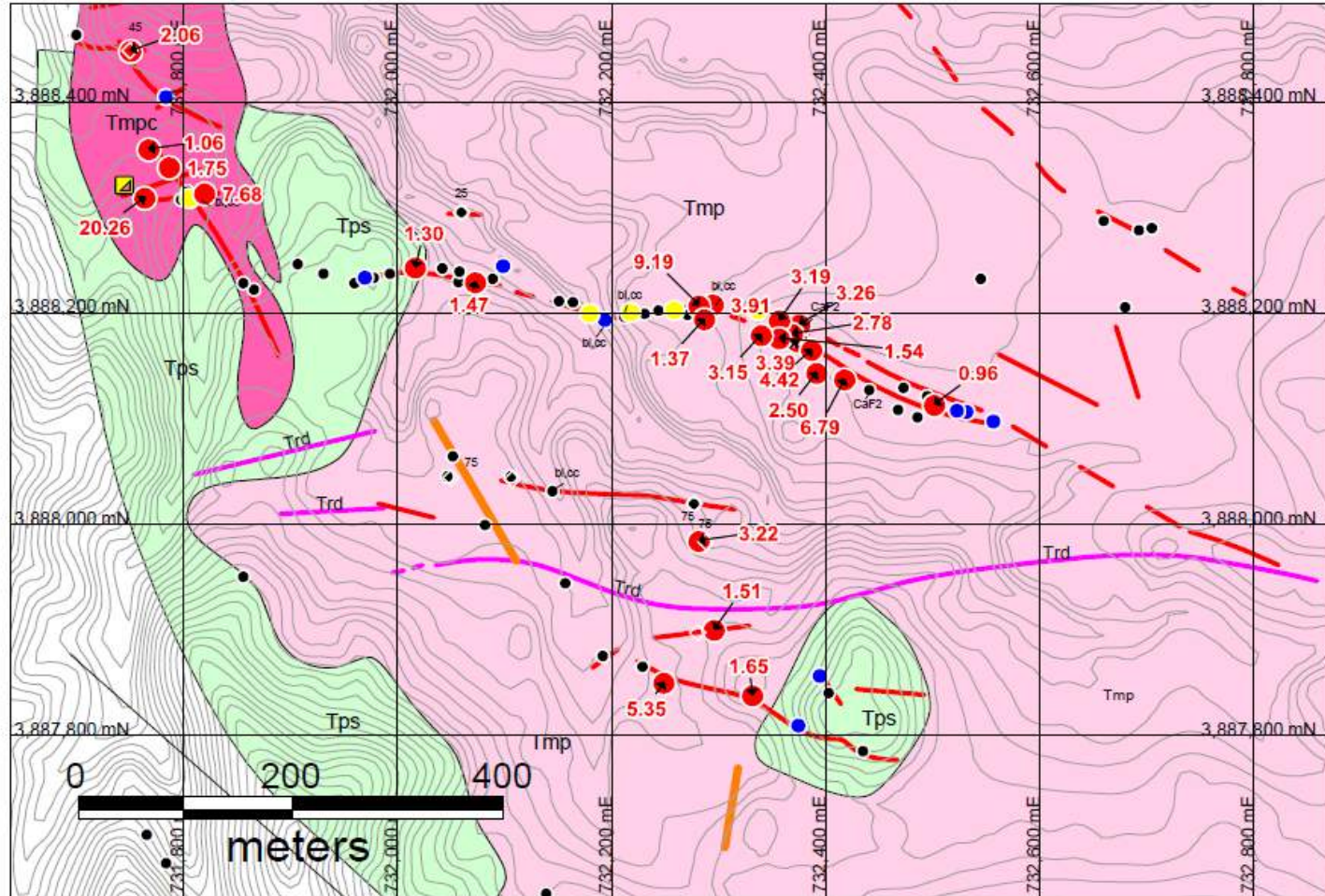
Fig. 3: Moss Property - Old Timer Area - Au in 2014 Rock Sampling
